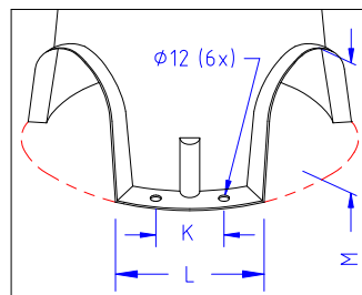
DETAIL BASE
