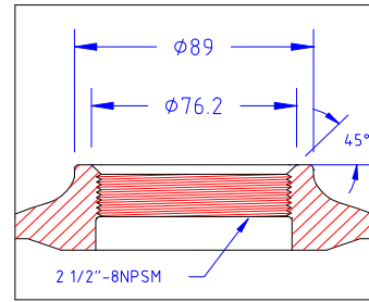
DETAIL 2 1/2" THREAD
